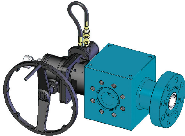
Model SCB Choke with Hydraulic Actuator and Manual Override
